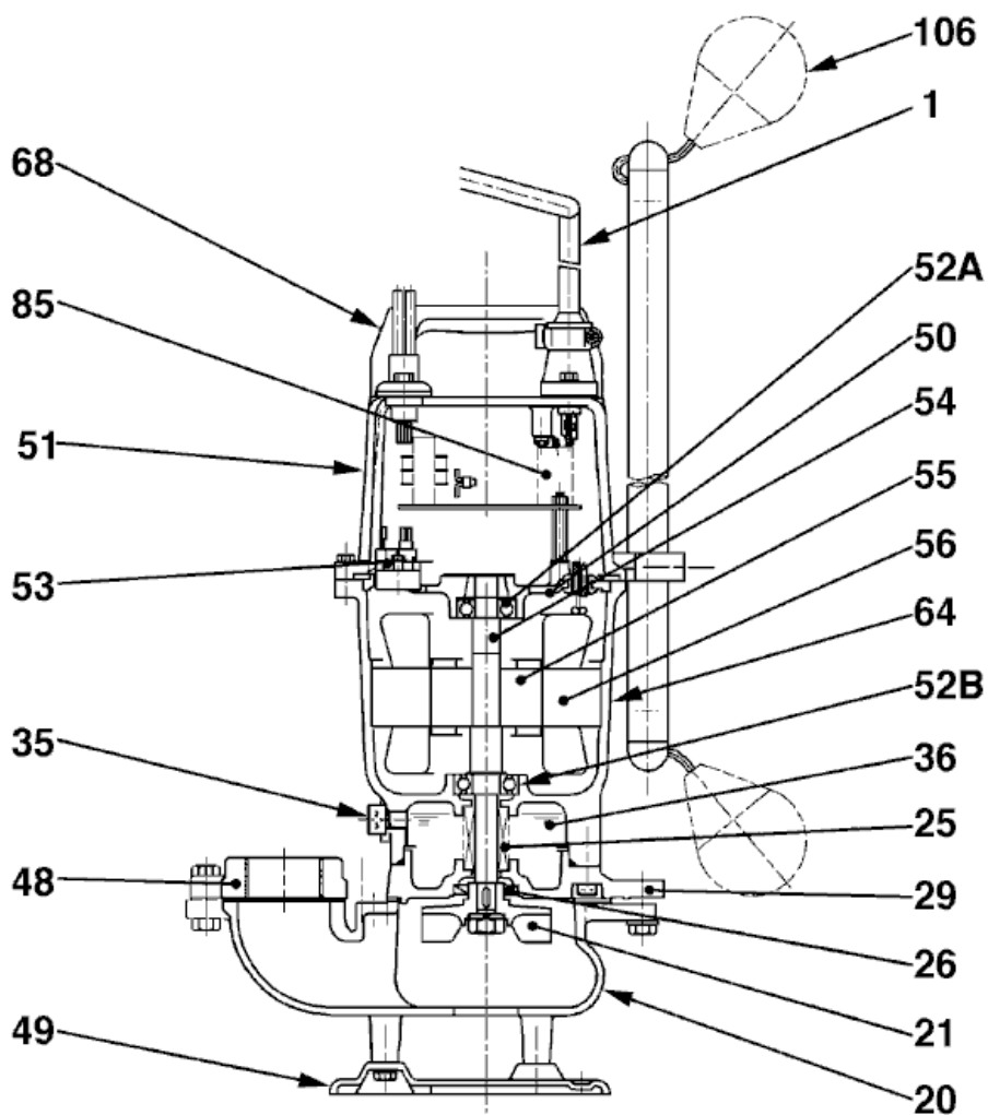
40UA2.25 (A-01997-2)
